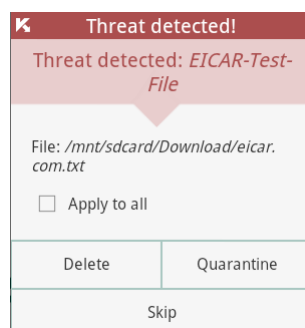
Figure 6. Notification windows
