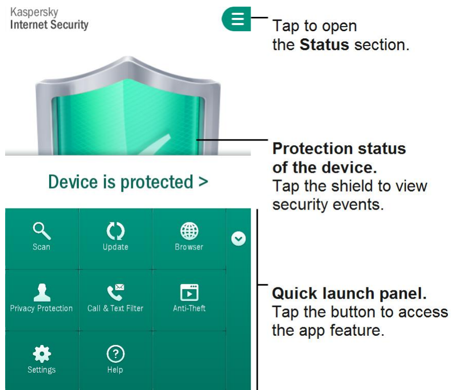
Figure 1. Main window
